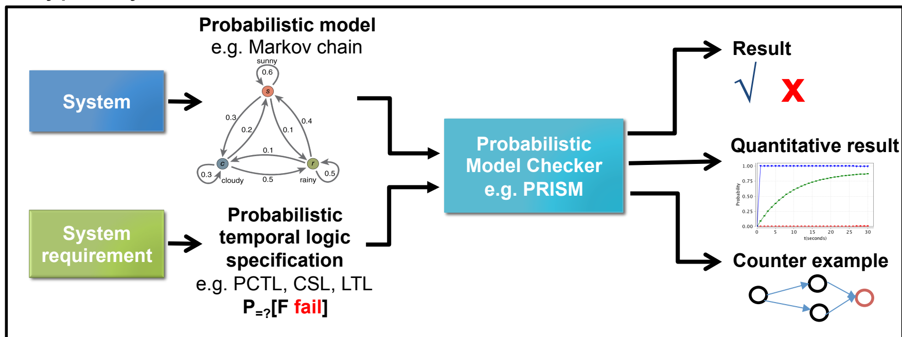
Figure 2. Probabilistic model checking
