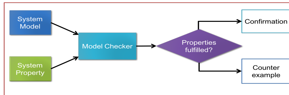
Figure 1. Model checking
