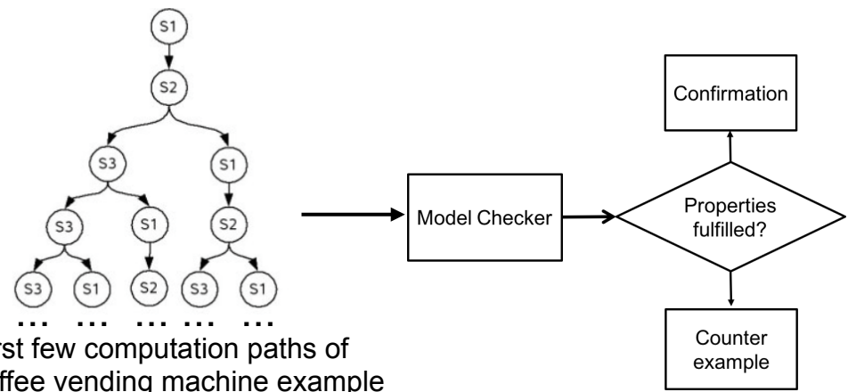
Figure 1. Model checking
