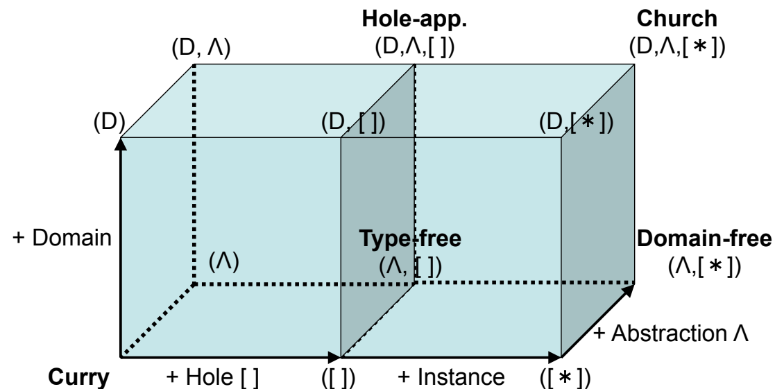
Figure 3: \lambda^2 -terms with fine structures between Curry-style and Church-style
